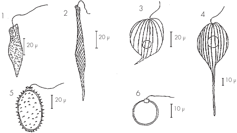
Fig. 10 – Phytoplancton (Planche 4/5).
