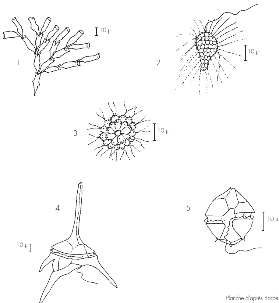
Fig. 10 – Phytoplancton (Planche 2/5).
