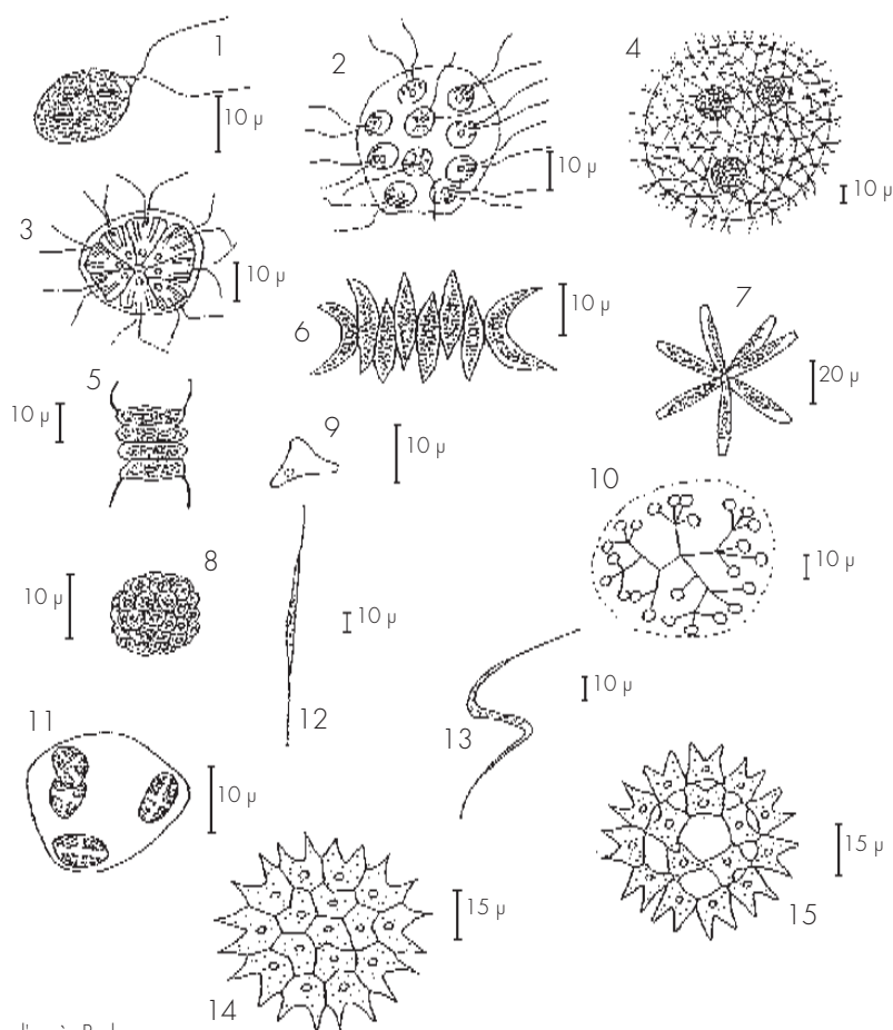
Fig. 10 – Phytoplankton (Planche 3/5).
